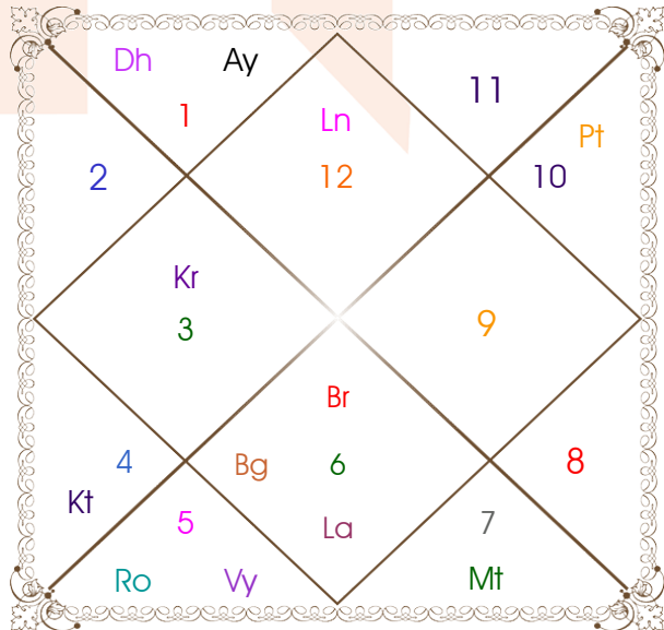
Arudha Chart
