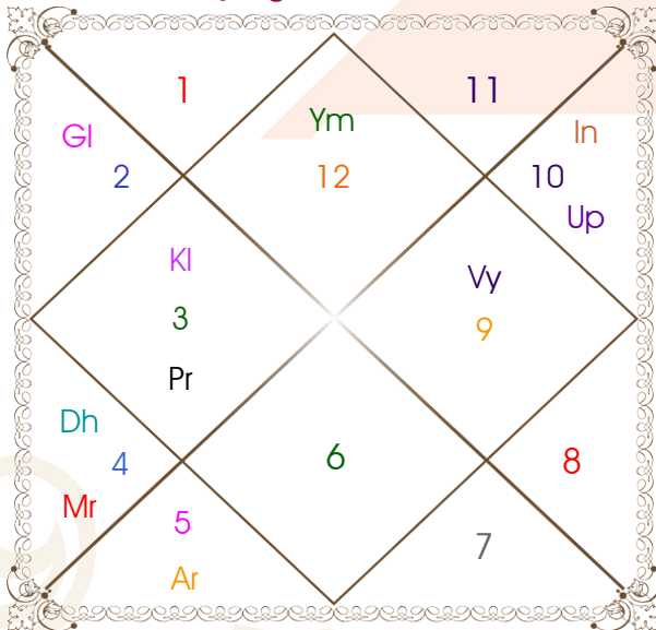
Upagraha Chart
